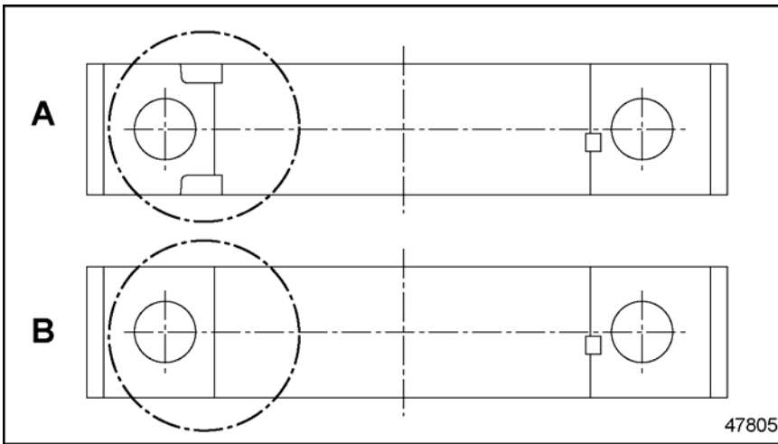
Figure 1 Main Bearing Cap Ends Showing Machined Notches and No Notches
